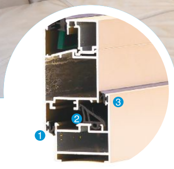
Triple Sealing
